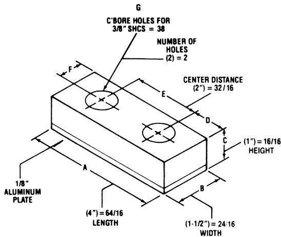
ERB-1540 60 Durometer Neoprene
