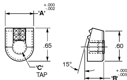
EFSC-127-4 SHOWN
